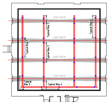
LOAD RAILS LOAD RATINGS HUNG FROM CONCRETE BEAMS REFER SHEET 2 FOR DETAILS
