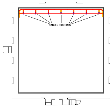
LADDER FRAME LOAD RATINGS HUNG FROM CEILING REFER SHEET 2 FOR DETAILS
