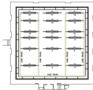
LIGHTING RAIL LOAD RATINGS GALLERY LEVEL (Level +21) REFER SHEET 2 FOR DETAILS
