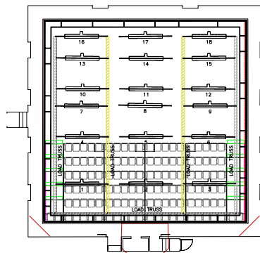
LOAD RAILS LOAD RATINGS HUNG FROM CONCRETE BEAMS REFER SHEET 2 FOR DETAILS
