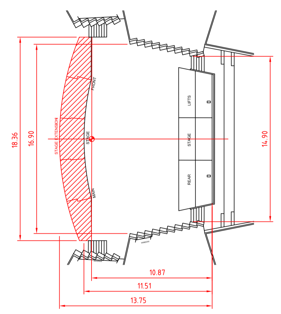
STAGE DIMENSIONS
