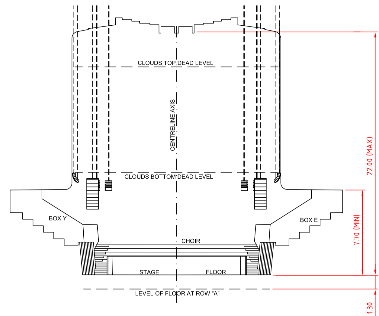
EAST-WEST SECTION
