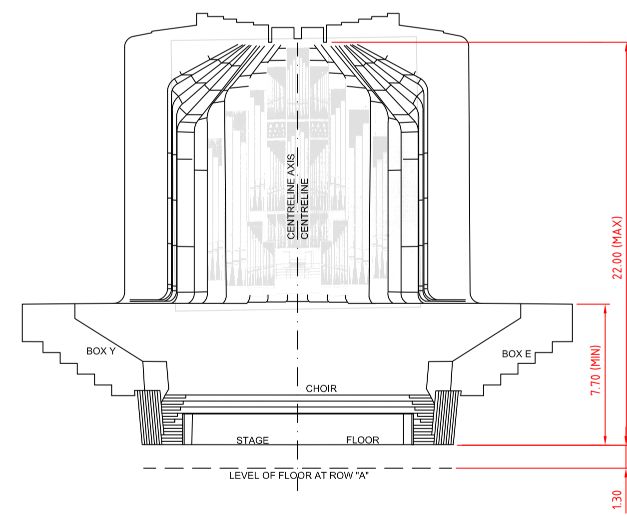
ORGAN ELEVATION
