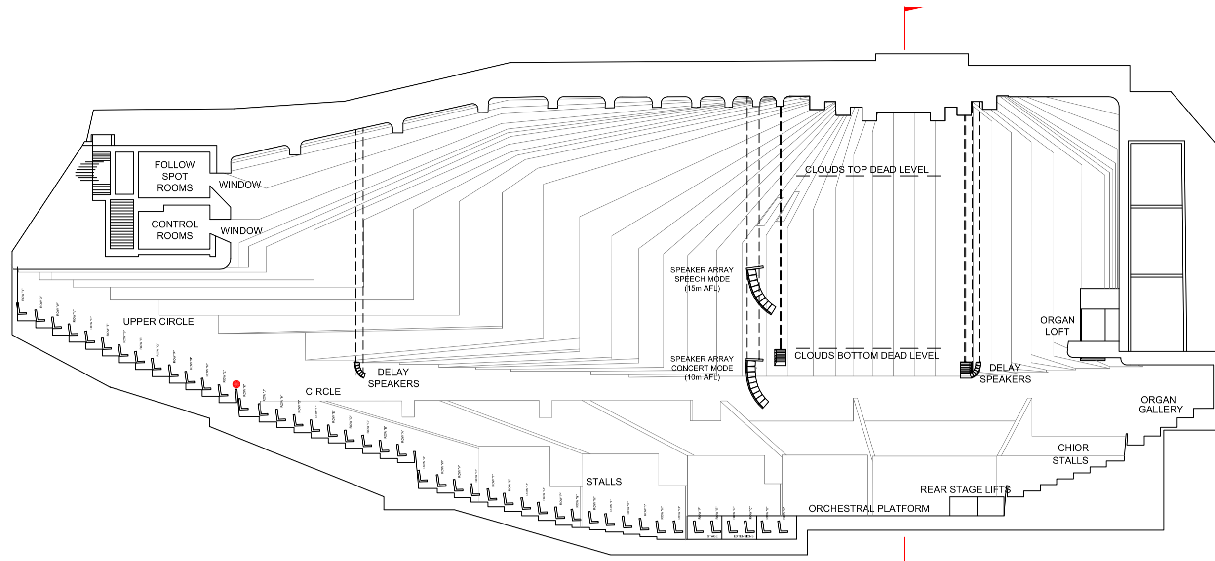
NORTH-SOUTH SECTION
